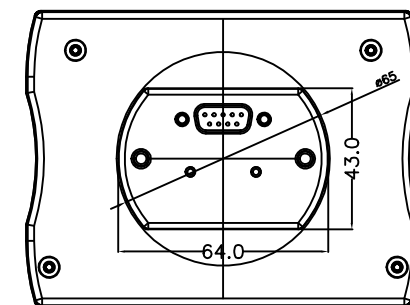
METER CUTTING HOLL (사각홀(64*43) 및 원형홀(65Φ))
