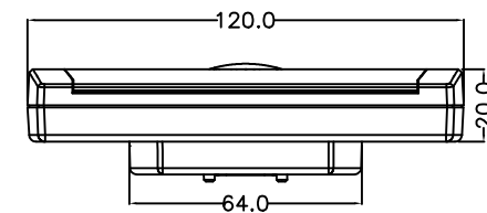
METER CUTTING HOLL (사각홀(64*43) 및 원형홀(65Φ))
